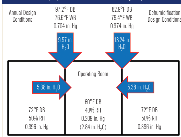
FIGURE 1 Potential vapor pressure differentials across building components of the OR.
